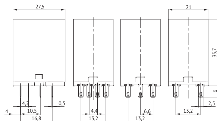
OptiRel G RP55-3X
