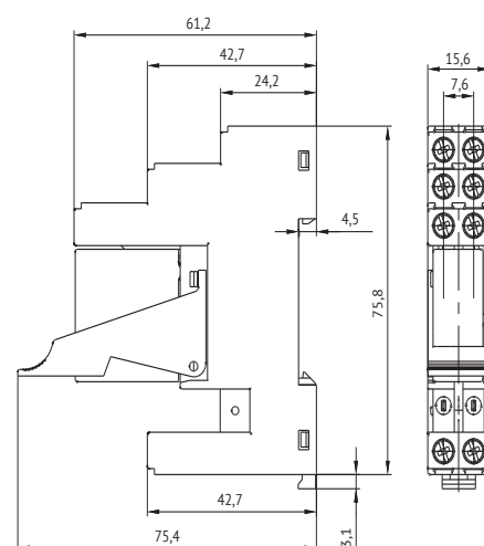
OptiRel G RM48
