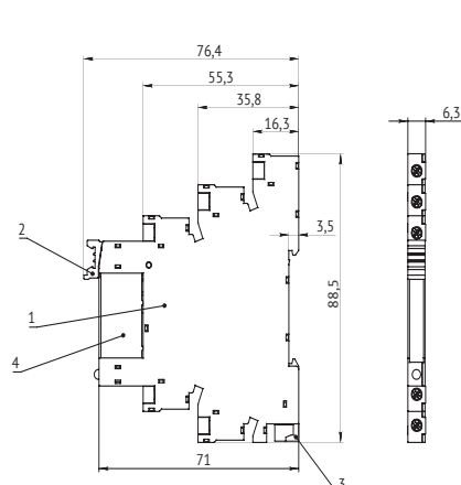
OptiRel G RM38
